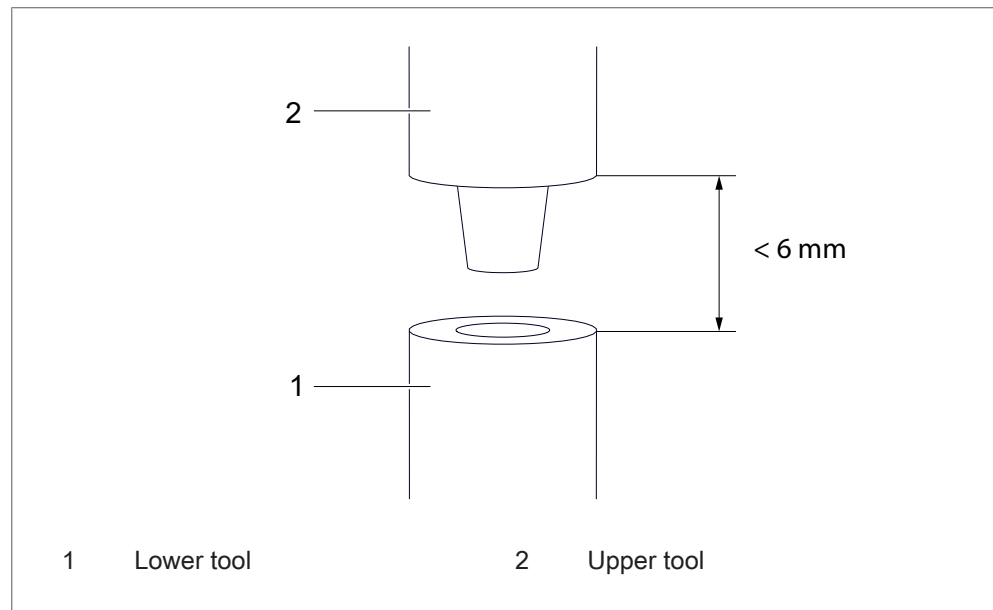
Fig. 4 Example: Tool opening pinch-off edge <math>< 6 \text{ mm}</math>
